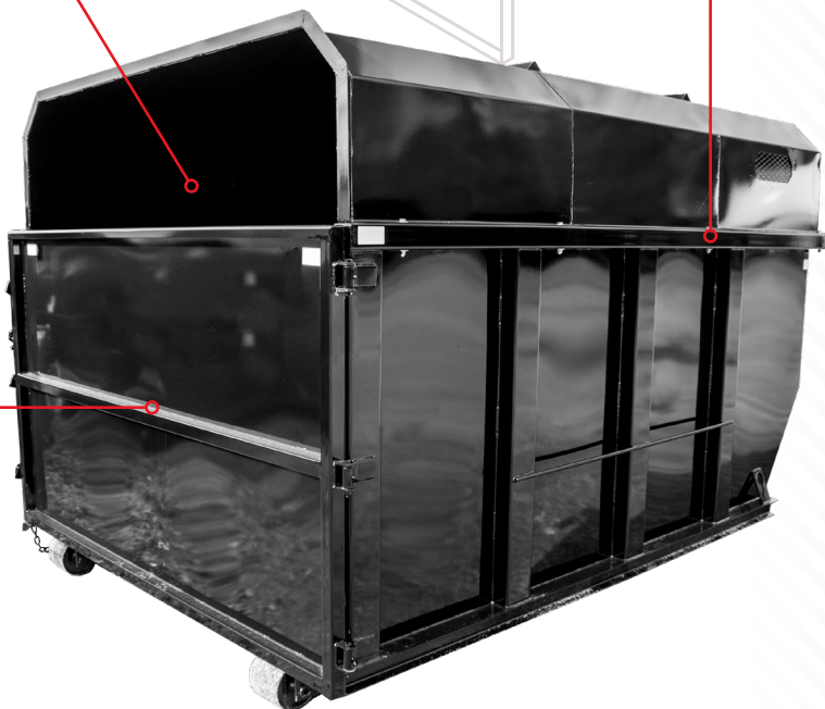
One Piece Roof bolted onto Arbor Body
